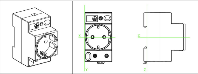
SB103148_CAD2D_Dimension
