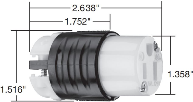
Dimensions for 15 & 20 Amp Connector
