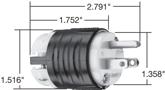
Dimensions for 15 & 20 Amp Plug
