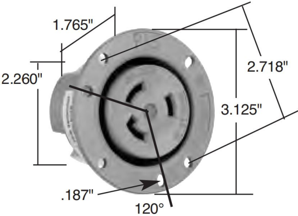
Dimensions for 30 Amp Flanged Outlet
