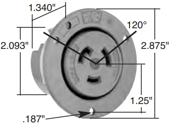
Dimensions for 20 Amp Flanged Outlet
