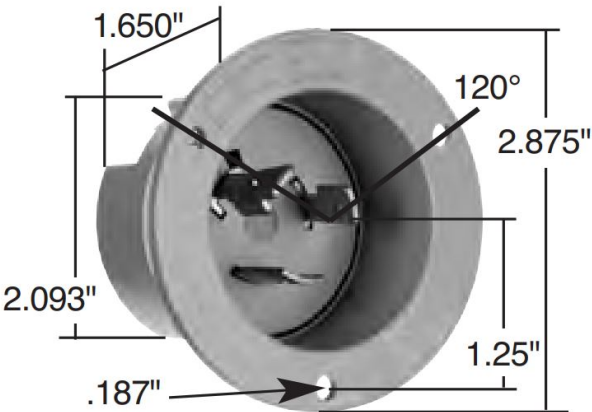
Dimensions for 20 Amp Flanged Inlet
