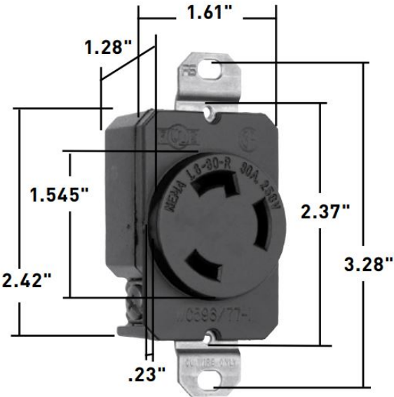
Dimensions for 30 Amp Receptacle
