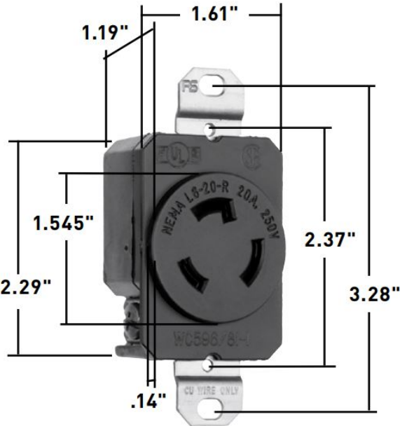
Dimensions for 20 Amp Receptacle
