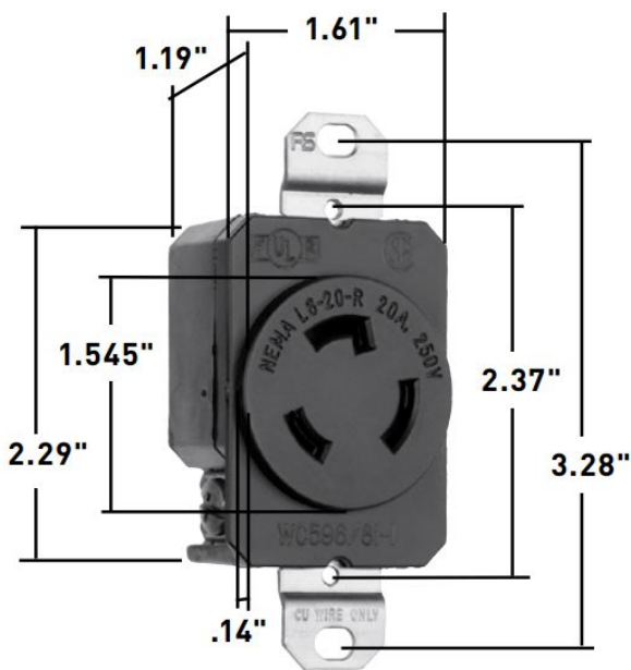
Dimensions for 20 Amp Receptacle
