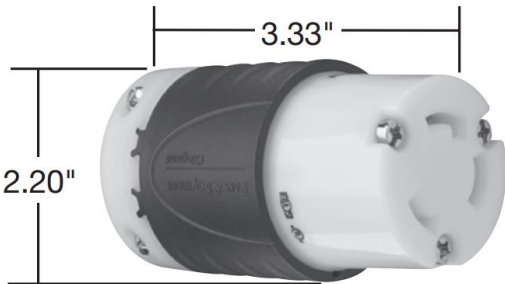
Dimensions for 20 & 30 Amp Connector
