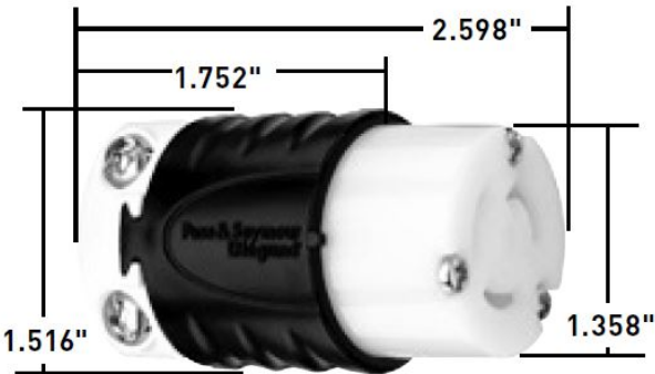
15A Connector
