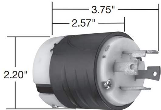
Dimensions for 20 & 30 Amp Plug
