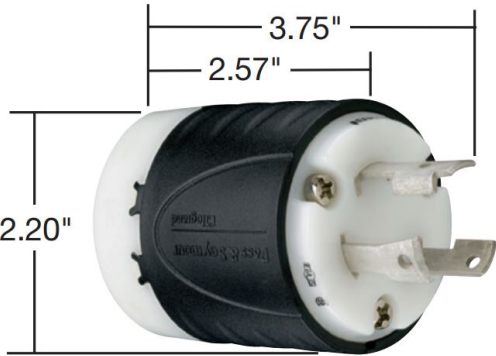
Dimensions for 20 & 30 Amp Plug
