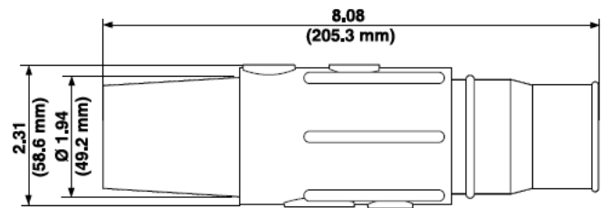
Female Plug - Double Set Screw Detachable
