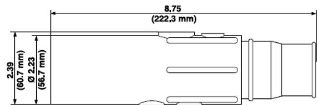
Male Plug – Double Set Screw Detachable
